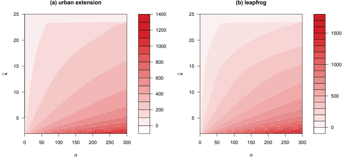
Figure 3: Effect of the AEP on the total contracted area S_a^*
