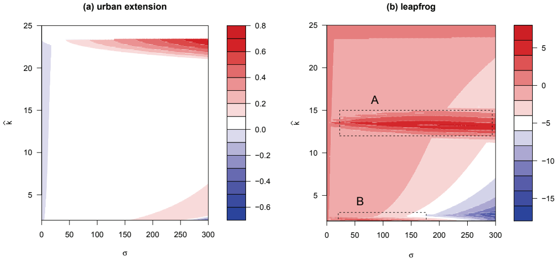
Figure 5: Effect of the AEP on (x_2 - x_1) + (x_4 - x_3) in %
