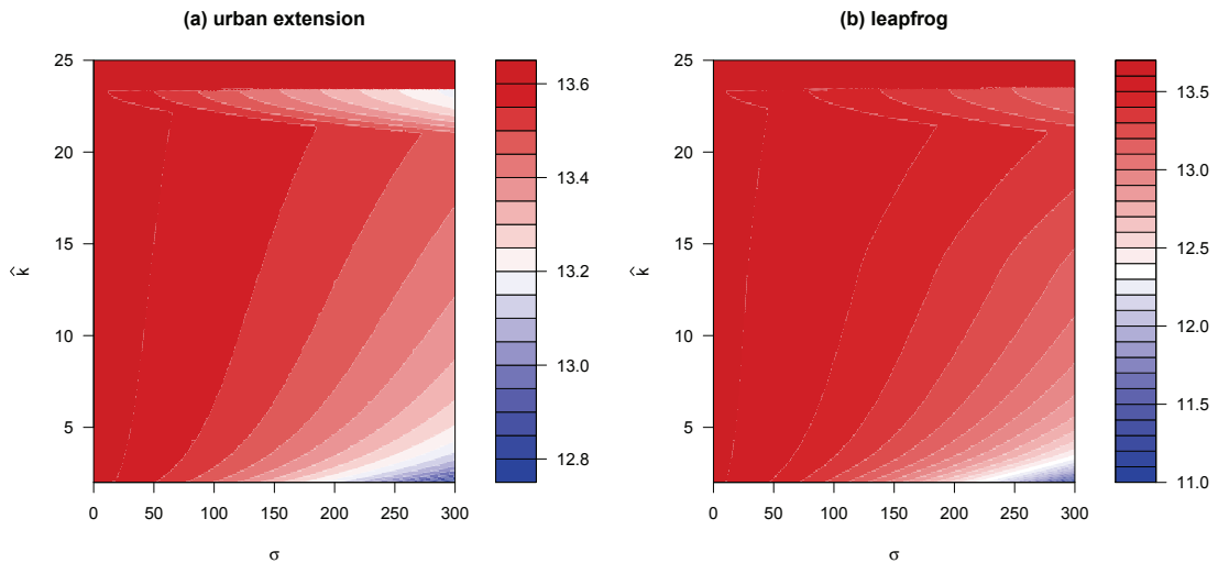
Figure 4: Effect of the AEP on \bar{x}
